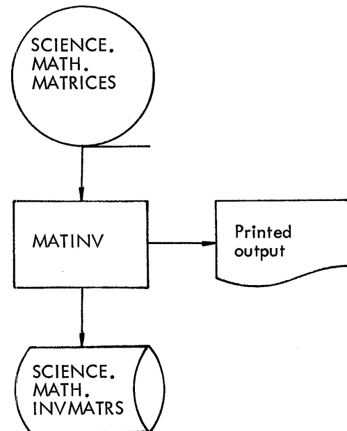
Figure 26. I/O flow for Example 1.
