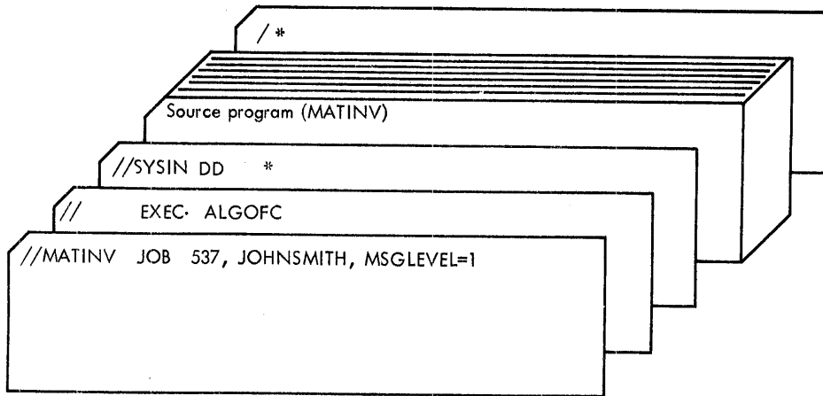
Figure 2. Sample deck for using ALGOFC cataloged procedure with a single source program. This job compiles the MATINV source program used in Example 1 of Appendix E.
