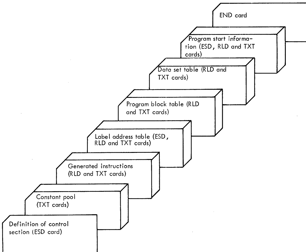
Figure 20. The object module card deck. The ESD (External Symbol Dictionary) cards contain the external symbols that are defined or referred to in the module. The RLD (Relocation Dictionary) cards contain addresses used in the module. The TXT (Text) cards contain the constants and instructions used in the module. The END card indicates the end of the module.
