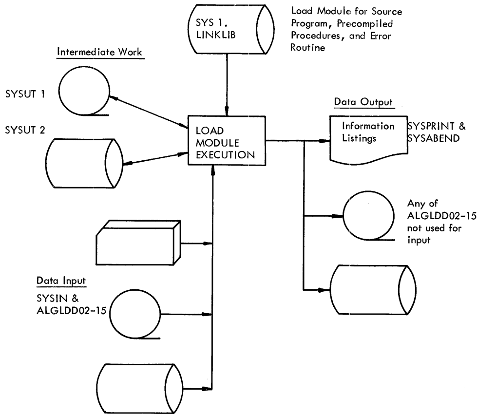
Figure 9. Flowchart showing data sets used at load module execution. The data input and output requirements are variable.
