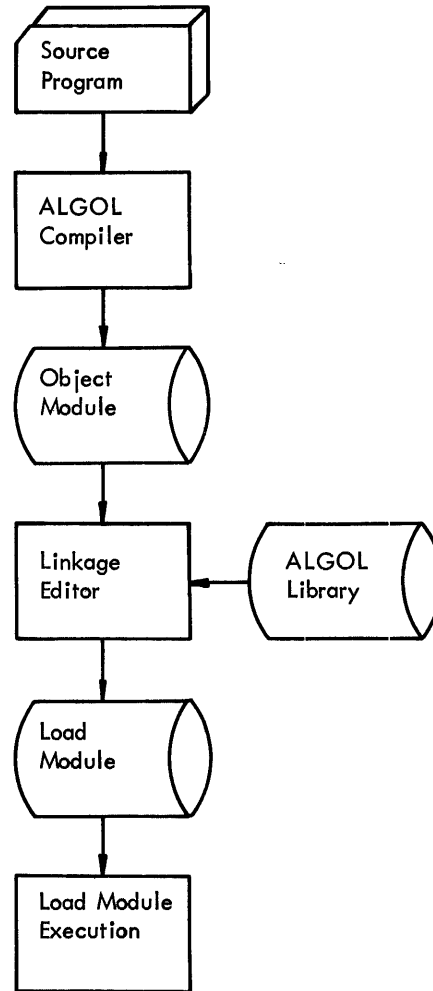
Figure 1. Basic flowchart for handling an ALGOL program.
