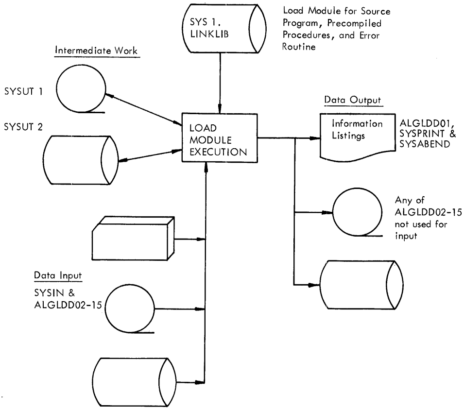
●Figure 9. Flowchart showing data sets used at load module execution. The data input and output requirements are variable.
