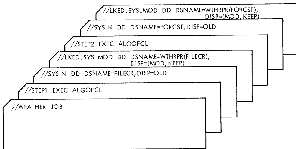
Figure 3. Sample deck for using ALGOFCL cataloged procedure with two source programs. These two job steps compile and linkage edit the two source programs used in Example 3 of Appendix E. Both source programs have been previously stored on intermediate I/O devices.
