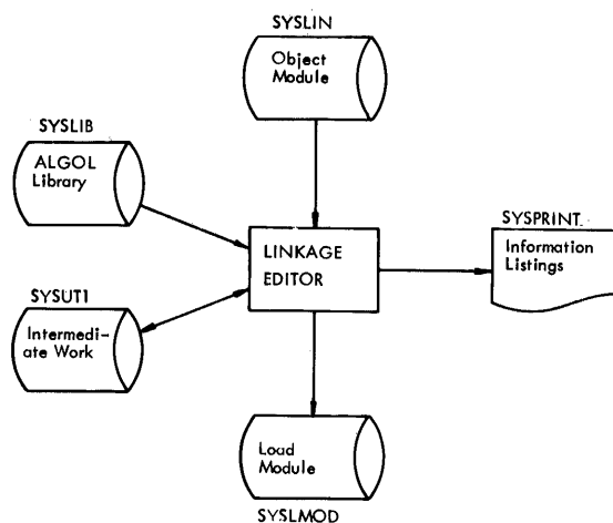
•Figure 7. Flowchart showing data sets used by the linkage editor.
