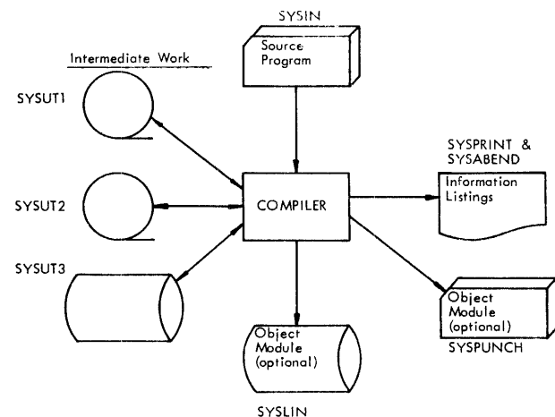
Figure 4. Flowchart showing data sets used by the compiler.
